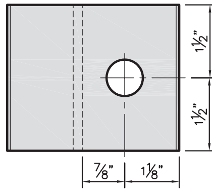
1 Hole Clamp
