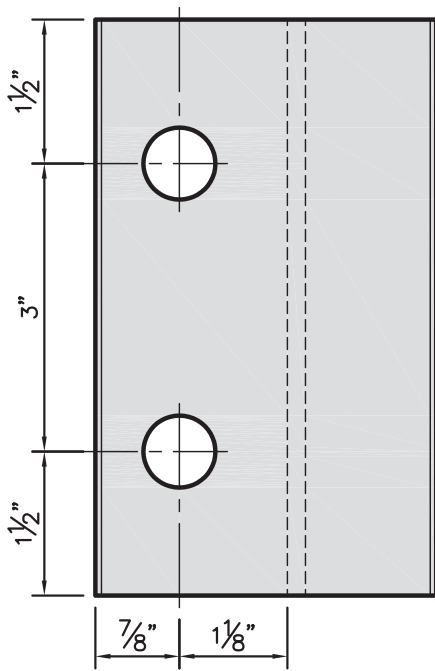
2 Hole Clamp
